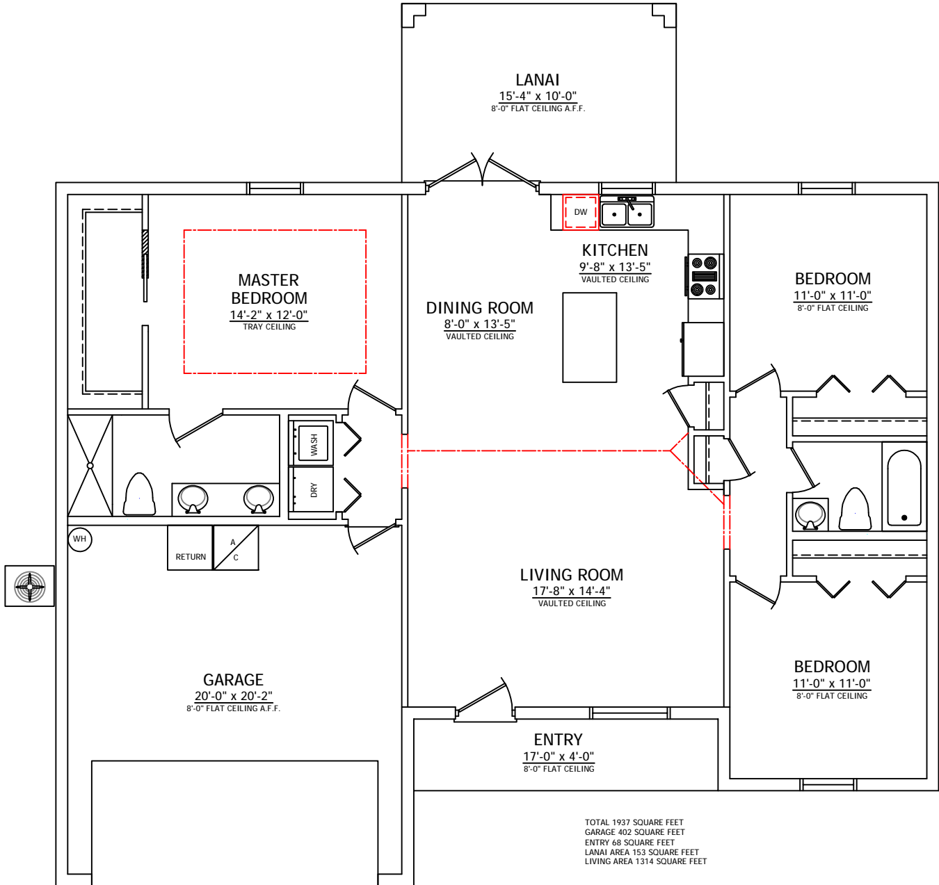
FLOOR PLAN
