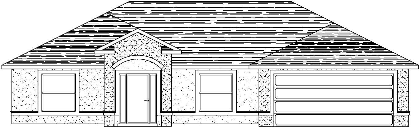
FRONT ELEVATION
